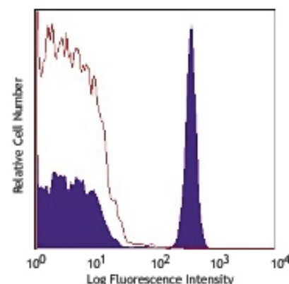
Human peripheral blood lymphocytes stained with SK3 APC/Cy7
