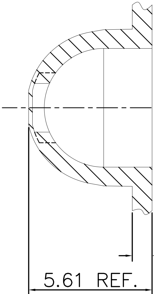
SECTION X-X
